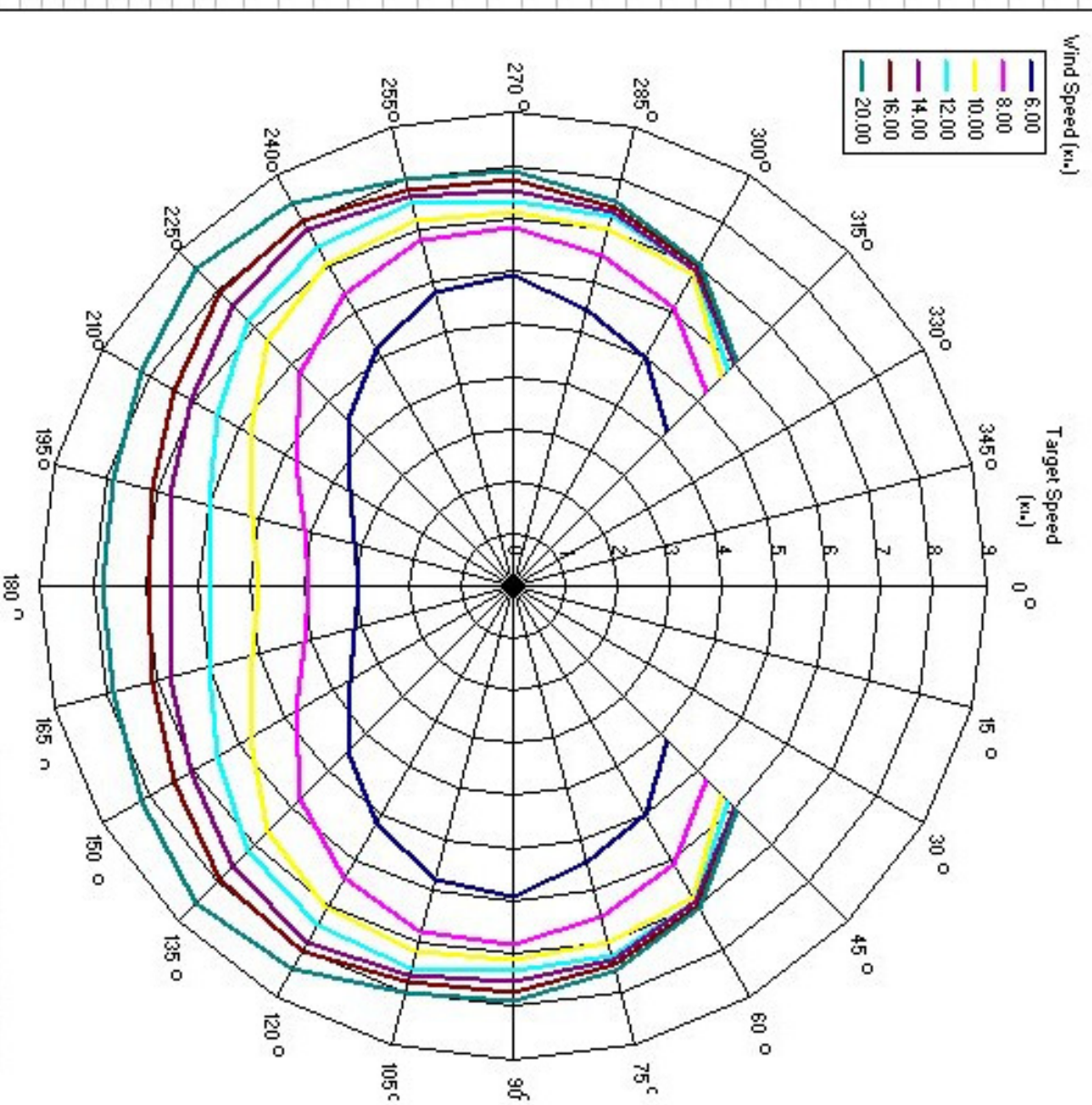
Catalina 320 Polar Plot
